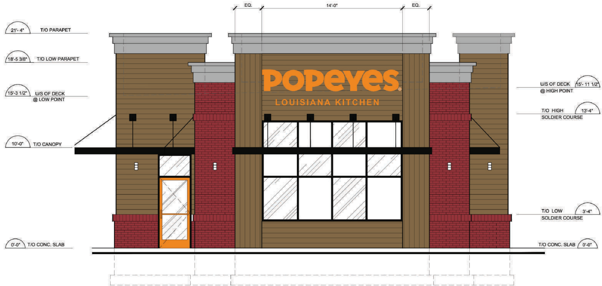
1 PROPOSED FRONT ELEVATION A5 SCALE: 1/4"=1' - 0"
